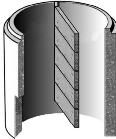
Section View Showing Treated Lumber Boards
